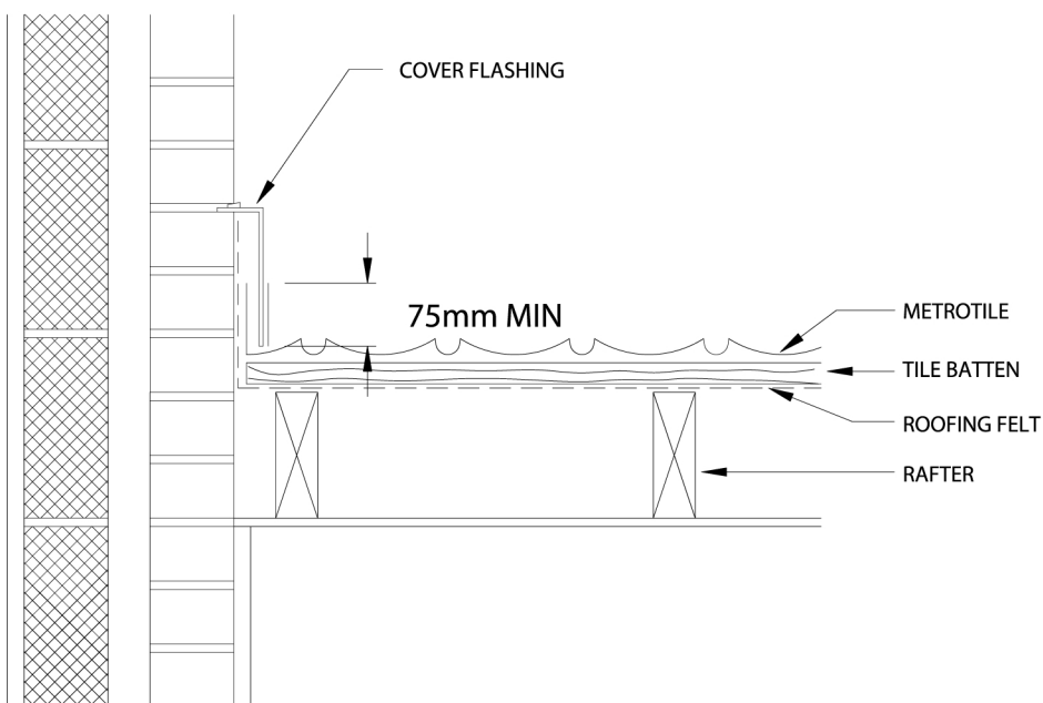
ALTERNATIVE DETAIL WITHOUT SIDEWALL FLASHING
