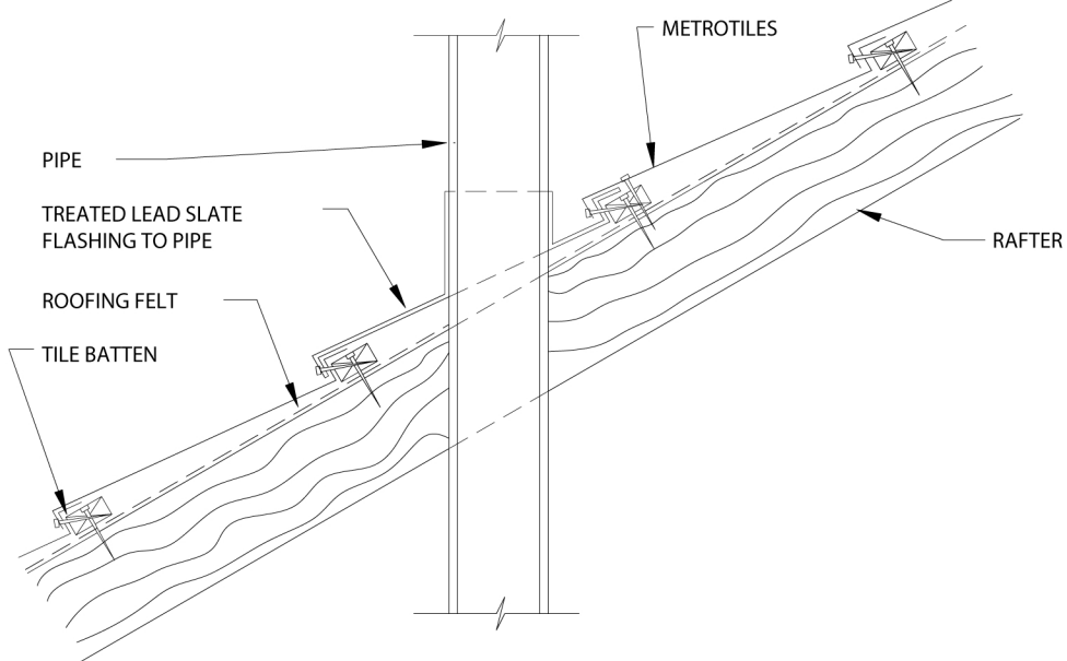
SOIL VENT PIPE THROUGH ROOF
