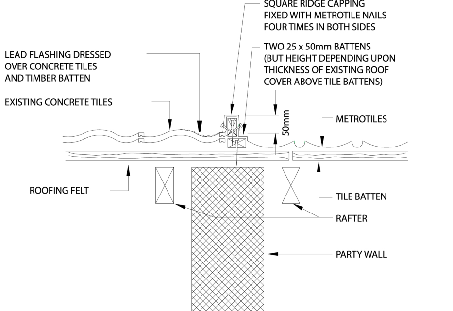
DETAIL OF METROTILES ABUTTING CONCRETE TILES OF PROFILED SECTION
