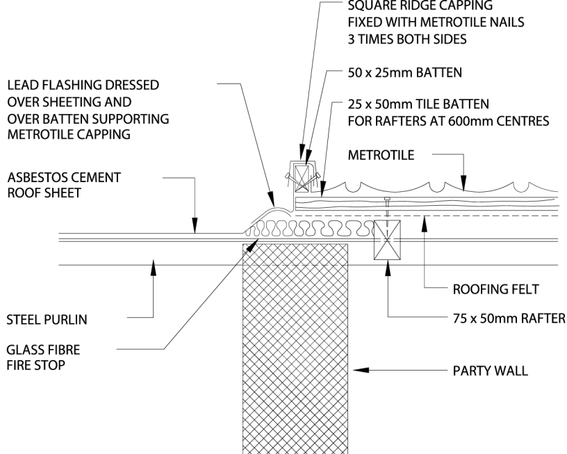
DETAIL OF METROTILE ABUTTING ASBESTOS SHEETS
