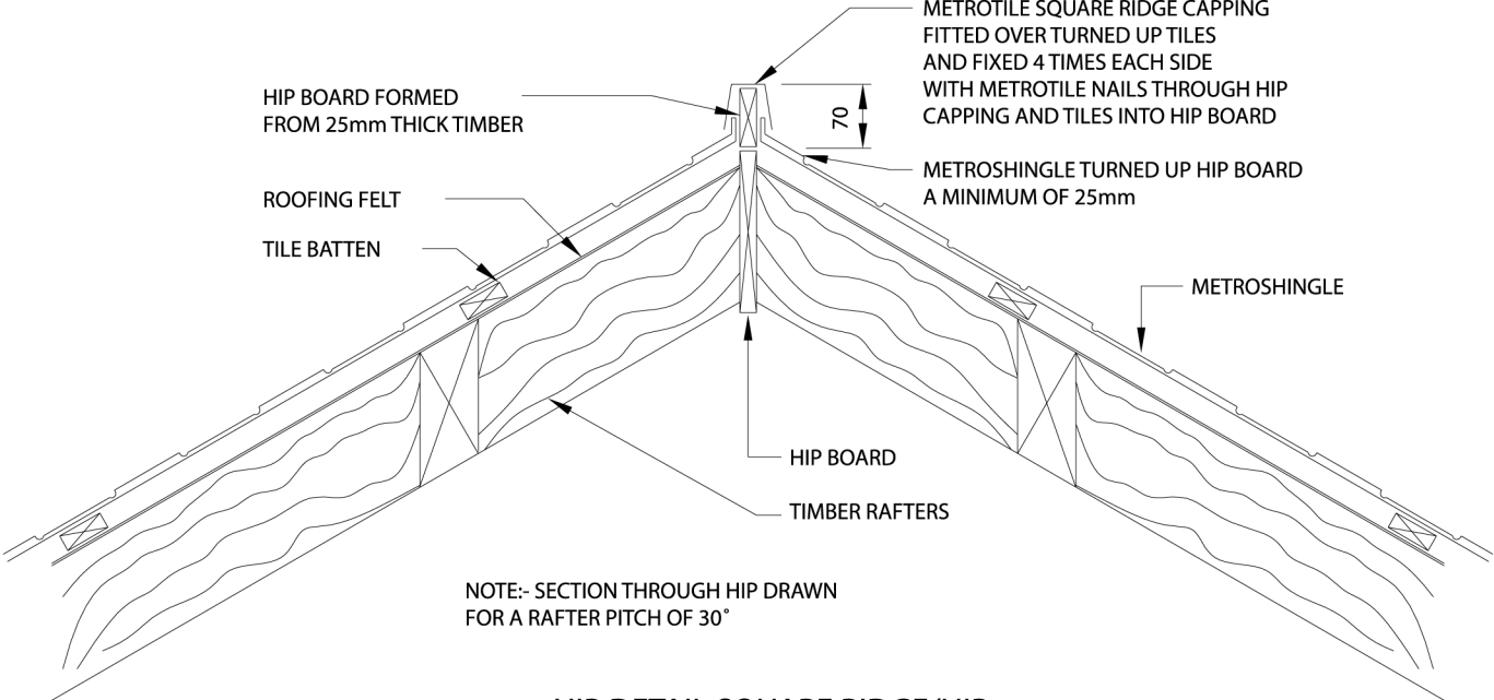
HIP DETAIL SQUARE RIDGE/HIP
