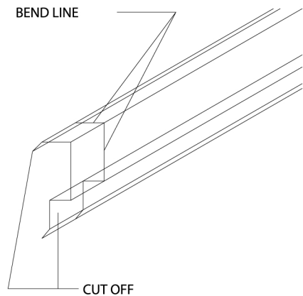
ENLARGED DETAIL OF END OF BARGE
